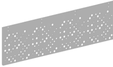
THRESHOLD MPS1300 L: 1298 mm / 51.10 inch D: 1,5 mm / 0.59 inch H: 357 mm / 14.05 inch
