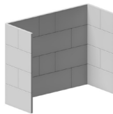
MEGARON PANEL SO H4U01 L: 2100 mm / 82.68 inch D: 850 mm / 33.46 inch H: 1625 mm / 63.98 inch
