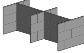
MEGARON S0 MCCPNL_H3_H4 L: 3350 mm / 131.89 inch D: 1600 mm / 62.99 inch H: 1225 mm / 48.23 inch
