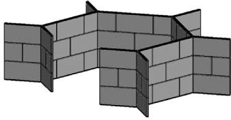
MEGARON S0 MCCPNL_H3_P15 L: 4230 mm / 166.54 inch D: 3665 mm / 144.29 inch H: 1225 mm / 48.23 inch
